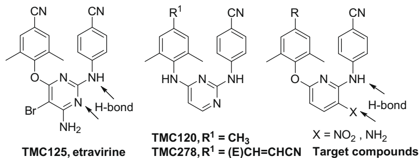
Figure 1. TMC125, TMC120, TMC278, and target compounds.
