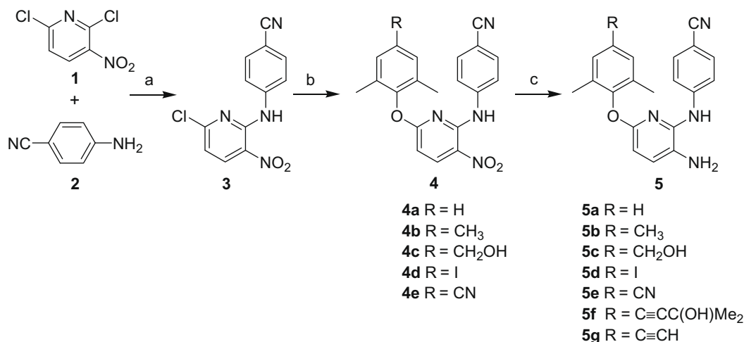
Scheme 1. Reagents and conditions: (a) 140 °C, 4 h, \text{N}_2 , 73%; (b) substituted phenol, \text{K}_2\text{CO}_3 , DMF, 120 °C, 6 h, 65–82%; (c) \text{Na}_2\text{S}_2\text{O}_4 , \text{NH}_3\cdot\text{H}_2\text{O} , \text{THF}/\text{H}_2\text{O} = 1/1 (v/v), rt, 3 h, 41–70%.
