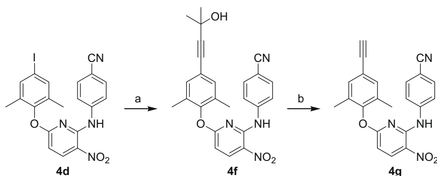
Scheme 2. Reagents and conditions: (a) 2-methyl-3-butyn-2-ol, \text{Pd}(\text{PPh}_3)_2\text{Cl}_2 , \text{Et}_3\text{N} , \text{CuI} , DMF, \text{N}_2 , rt, 7 h, 78%; (b) \text{NaOH} , toluene, reflux, 16 h, 69%.
